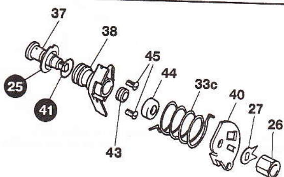
Early Alternative Starter Assembly
